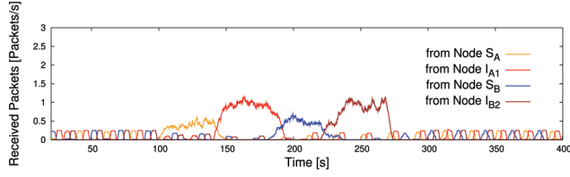
Fig. 4: WiseMAC: Packet Reception Rate from Nodes S_A , I_{A1} , S_B and I_{B1} .
