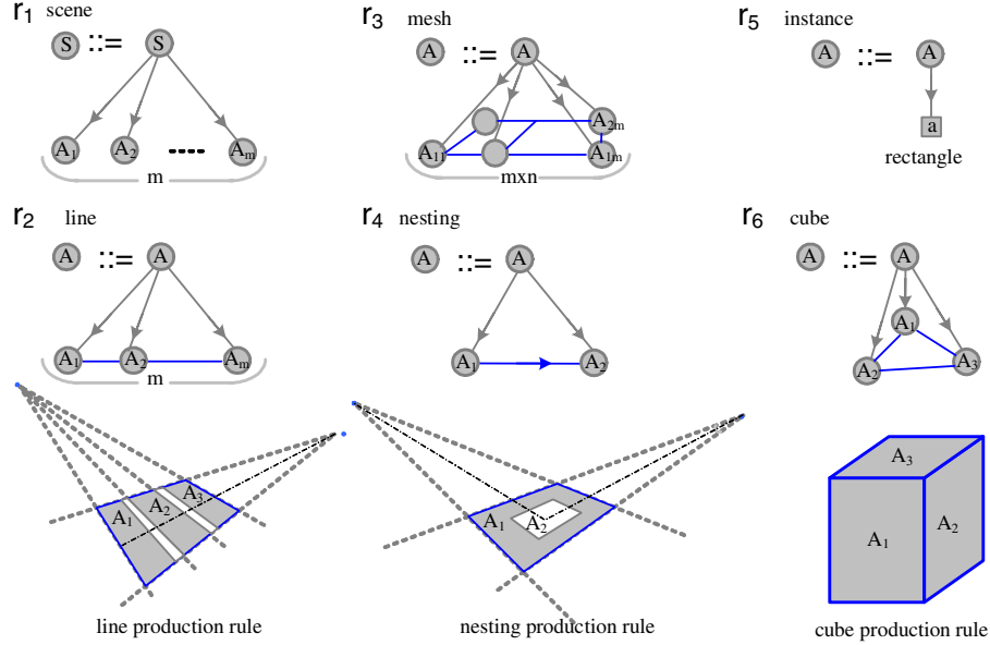
Fig. 9.1 Six attribute grammar rules for generic man-made world scenes. This grammar features a single class of primitives — rectangle and four generic organizations — line, mesh, cube, and nesting. Attributes will be passed between a node to its children and the horizontal lines show constraints on attributes. See text for explanation.
