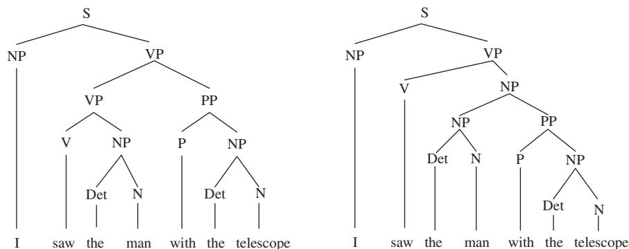
Fig. 2.6 An example of ambiguous sentence with two parse trees. The non-terminal nodes S, V, NP, VP denotes sentence, verbal, noun phrase, and verbal phrase, respectively. Note that if the two parses are merged, we obtain a graph, not a tree, with a “diamond” in it as above.
