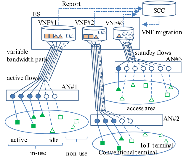
Fig. 6 Schematics of active flows and idle flows.
