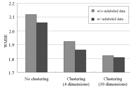
Fig. 3 Comparison of WMSE (6).
