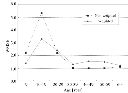
Fig. 4 WMSE for each age-group.
