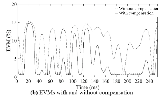
Fig. 7 Simulated EVM for Rayleigh faded channel ( f_D : 30 Hz).
