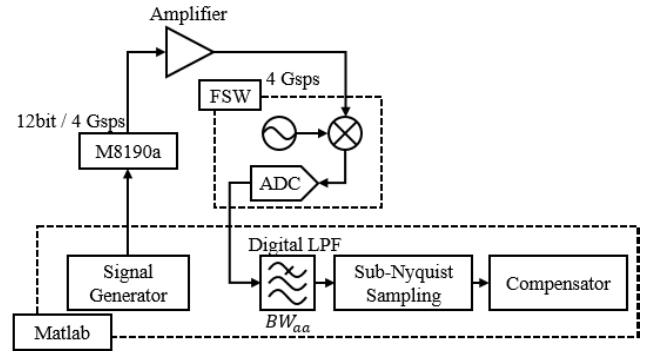
Fig. 12 Block diagram of experimental setup.
