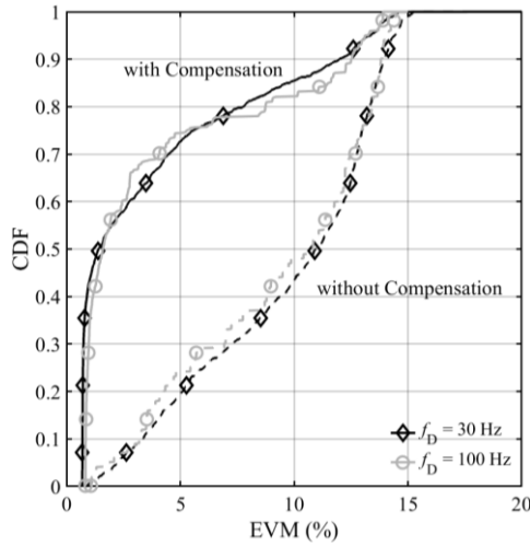
Fig. 8 CDF of EVM for Rayleigh Faded Channel ( f_D = 30, 100 Hz).
