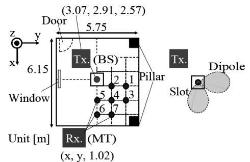
Fig. 14 Measurement environment.
