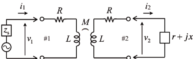
Fig. 1 Symmetric transformer circuit scheme
