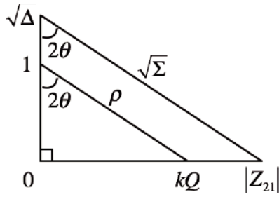
Fig. 6 Graphical visualization of Eqs. (74) and (76)
