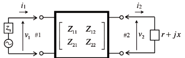
Fig. 5 Two-port black box for general formulation
