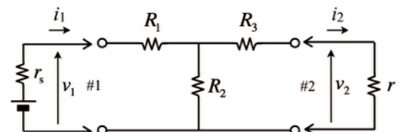
Fig. 4 T-shape resistive network
