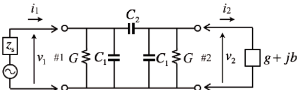
Fig. 3 \pi -shape capacitive network
