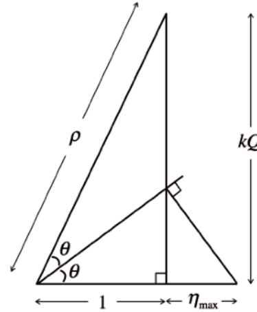
Fig. 7 Graphical visualization of Eqs. (75) and (77)
