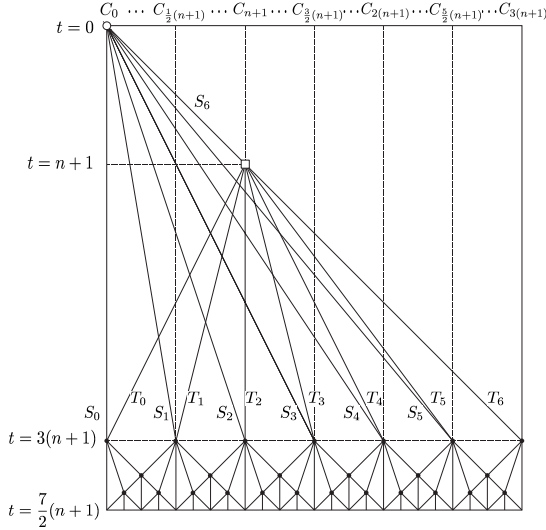
Fig. 10 Time-space diagram of the FSSP algorithm for a segment array when h = 3 , \alpha = 2 .
