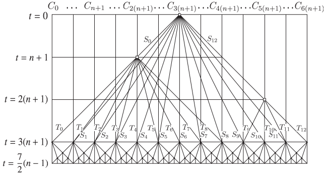
Fig. 12 Time-space diagram of FSSP algorithm for number pattern 0 when \alpha = 2 .
