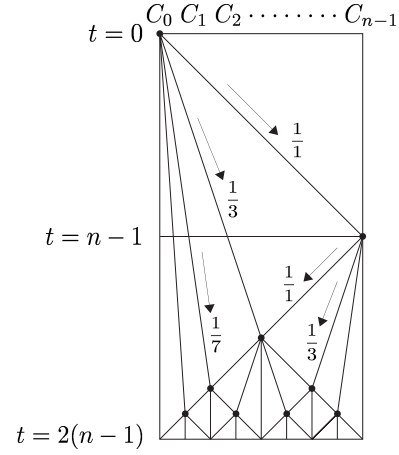
Fig. 1 Time-space diagram of a minimal time solution.
