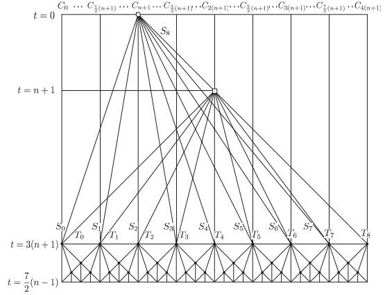
Fig. 11 Time-space diagram of the FSSP algorithm for number pattern 7 when \alpha = 2 .
