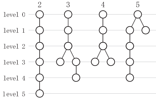
Fig. 6 Trees for number patterns 2, 3, 4 and 5.
