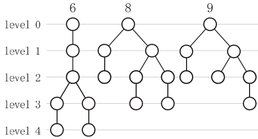
Fig. 8 Trees for number patterns 6, 8 and 9.
