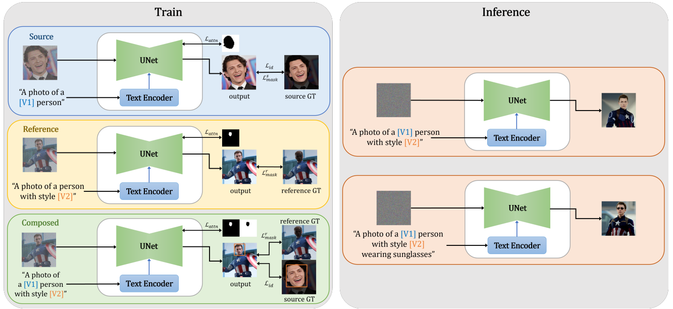
Figure 2: The overall pipeline of MagiCapture, where the training process is formulated as multi-task learning of three different tasks: source, reference, and composed prompt learning. In the composed prompt learning, reference style images serve as pseudo-labels, along with auxiliary identity loss between the source and predicted images. Attention Refocusing loss is applied to all three tasks. After training, users can generate high-fidelity images with integrated concepts and can further manipulate them using varying text conditions.
