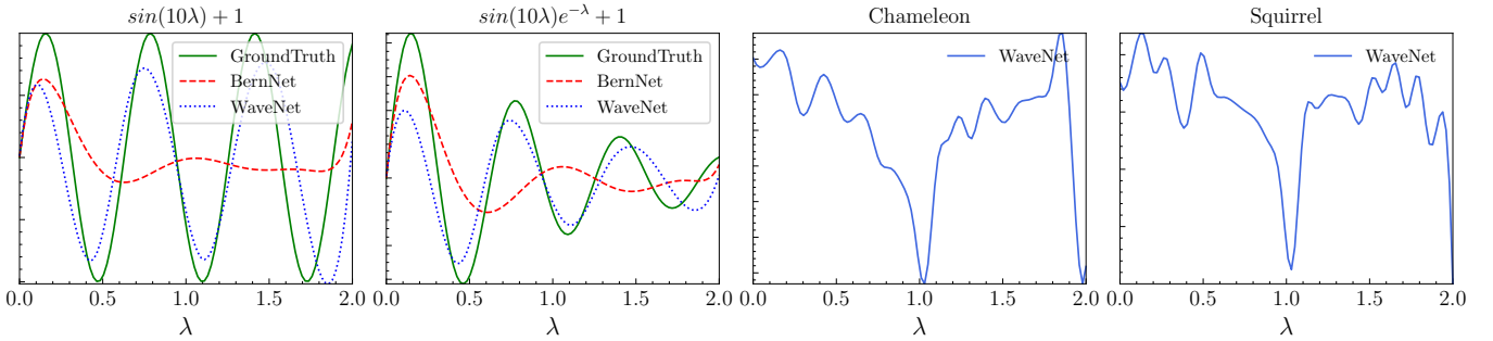
Figure 3: Left 2 Figures: Illustration of high-frequency spectral signals learned by BernNet and WaveNet. Right 2 Figures: Illustration of filters learned from real-world datasets by WaveNet.
