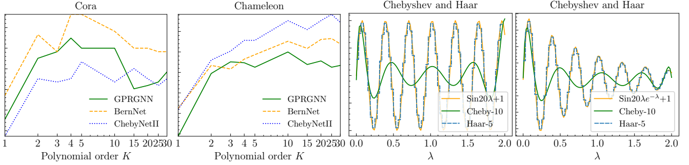
Figure 1: Left 2 Figures: Different polynomial order K applied to the Cora and Chameleon graph dataset. Mean accuracy is under 10 runs and the variance term is omitted. Right 2 Figures: The illustration about the ability of 10-order Chebyshev polynomial and 5-scale Haar wavelet to fit high-frequency signals, which are \sin 20\lambda + 1 and \sin 20\lambda \cdot e^{-\lambda} + 1 respectively.
