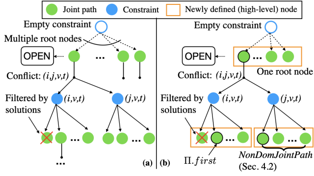
Figure 2: A conceptual visualization of MO-CBS and BB-MO-CBS.
