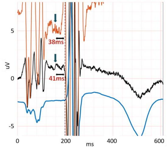
Figure 2: This figure shows Patient #25 filtered bipolar signal 3 (orange signal) and Laplacian signal 49 (black signal) with a bipolar non-invasive HV interval of 38 ms and Laplacian non-invasive HV interval of 41 ms (invasive HV measurement equals to 38 ms) superposed to lead V2 (blue signal).
