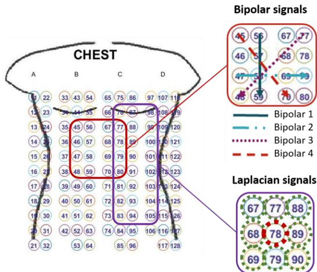
Figure 1: Chest electrode configuration. 24 Laplacian signals were created from the 128 body surface signals (bottom right) by subtracting the mean of the 8 neighbors (green dashed circle) from the central electrode signal (red dashed circle). Four bipolar signals were created (top right) in the 1. vertical, 2. horizontal, 3. right diagonal, 4. left diagonal directions.
