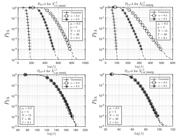
Fig. 3. P_{FA} - \lambda relationships for several parameters of the \mathcal{CCG} distribution.
