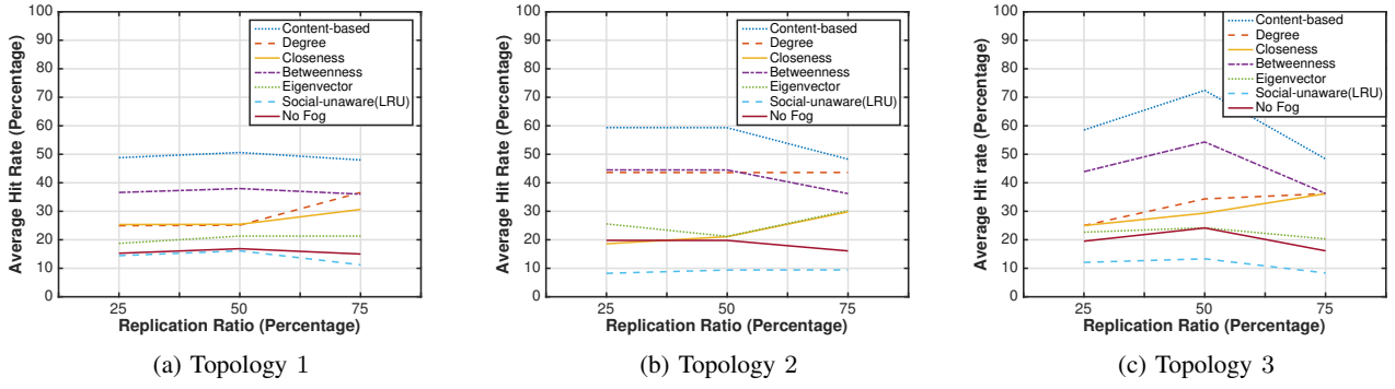
Figure 3: Hit rate comparison for centrality-based (CBC, Degree, Closeness, Betweenness, Eigenvector), non-centrality based or social-unaware (LRU) and non-collaborative (no fog) based caching.
