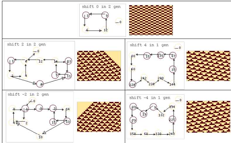
Figure 8. De Bruijn diagrams determining primitive gliders, periodic background, and other meshes (0,2), (4,1), (-4,1) in rule 54.
