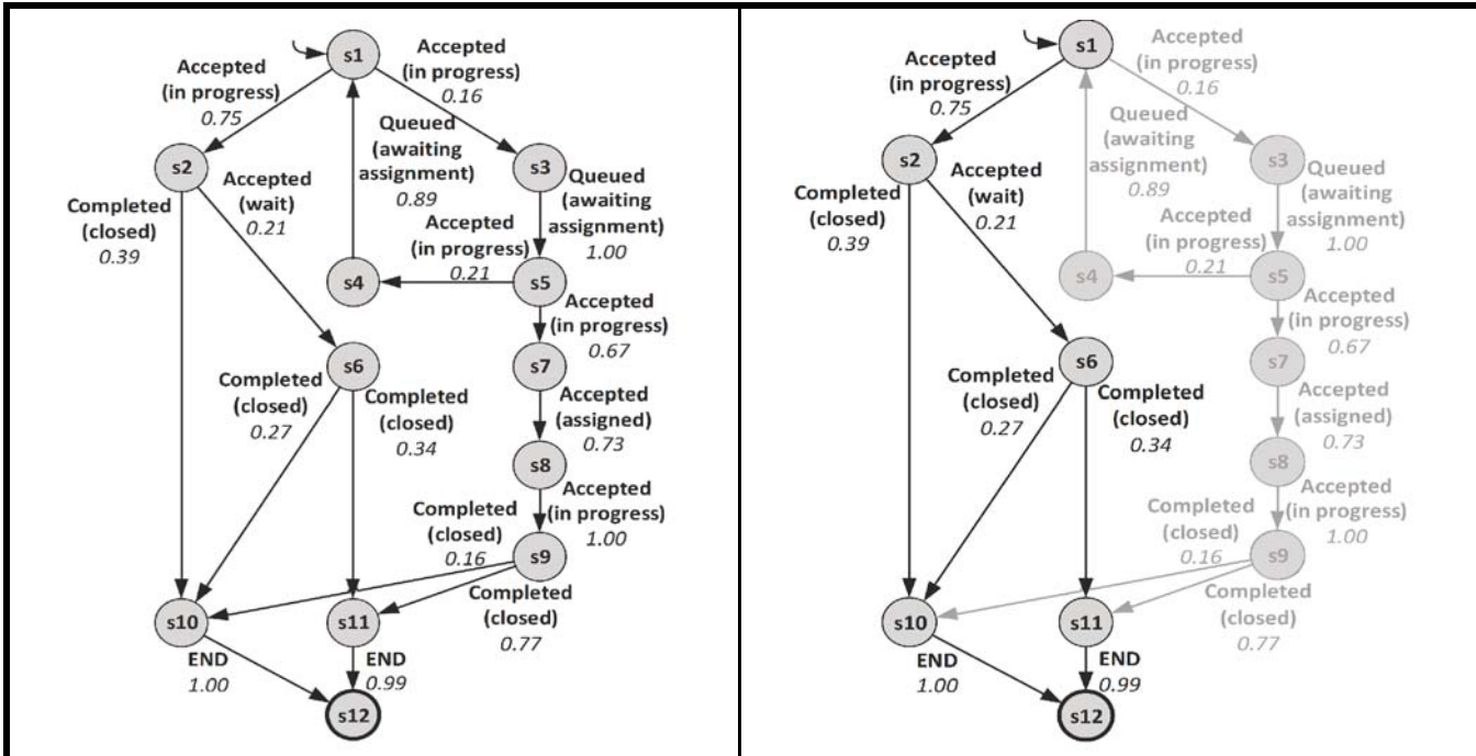
Figure 10. RegPFA Model Visualized with Abstraction Levels of \varepsilon = 0.1 (left) and \varepsilon = 0.2 (right)
