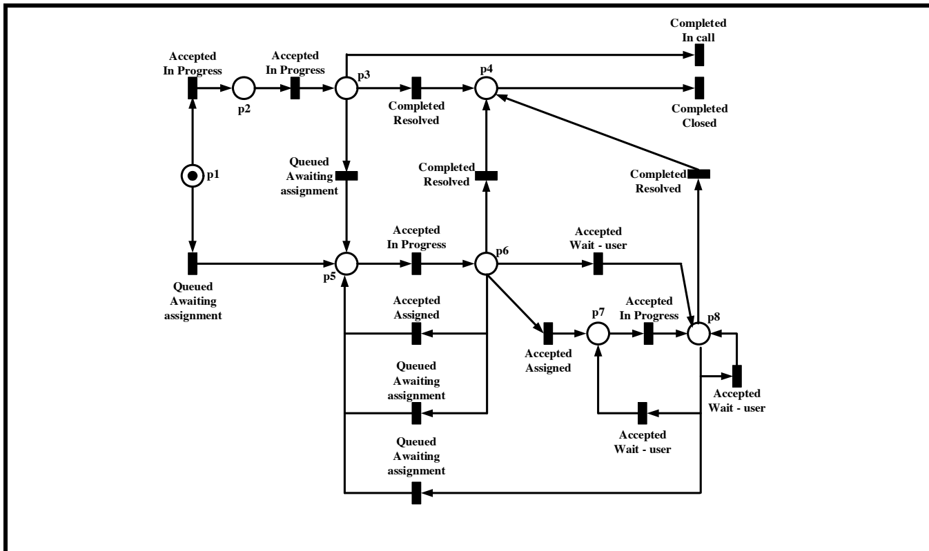
Figure 11. Petri Net Visualization of a Predictive Model for “BPI2013_Incidents”
