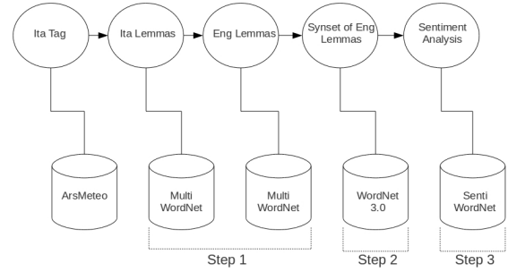
Fig. 2. Steps of the sentiment analysis on tags.
