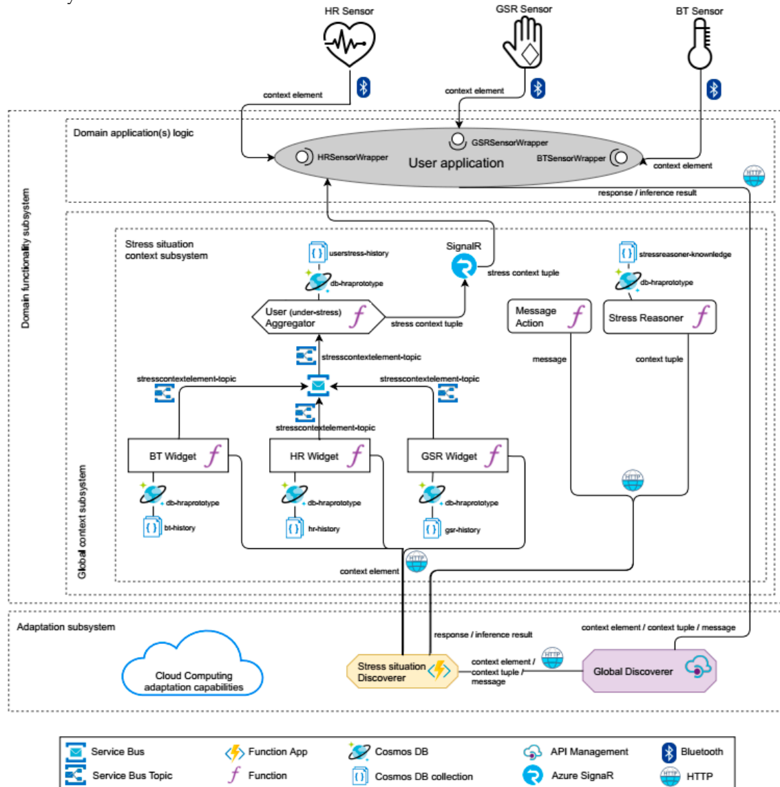
Figure 3. Detail of the prototype's deployment in Microsoft Azure using its serverless functions and services (only the stress situation context subsystem implementation is detailed).
