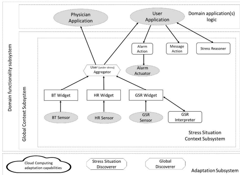
Figure 2. Stress situation context subsystem (adapted from [18]) of the global context subsystem as part of the redefined application layer by the proposed framework. BT: Body Temperature; HR: Heart Rate; GSR: Galvanic Skin Response.
