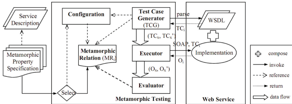
Figure 1. The framework of metamorphic testing for Web services
