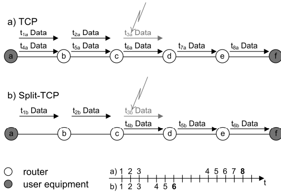
Figure 4: A packet is lost between router c and d. The duration t_{a8} until the retransmitted packet reaches the destination with TCP is much longer than t_{b6} with Split-TCP.
