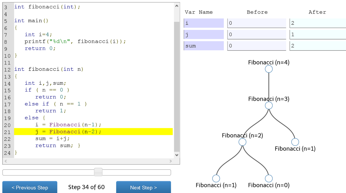
Figure 4: MindXpres source code plug-in example
