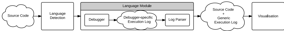
Figure 2: Architecture for extensible language support
