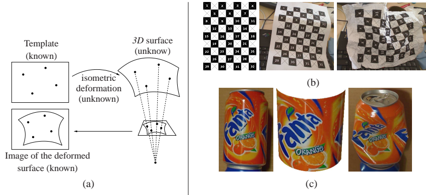
Figure 1: Monocular reconstruction of a deformable surface. (a) Problem setup. (b) Examples of paper sheets: the template (left) and two deformed sheets, a smooth one (middle) and a creased one (right). (c) Example of a can: template image (left), 3D template (middle), and the input image of the deformed can (right).
