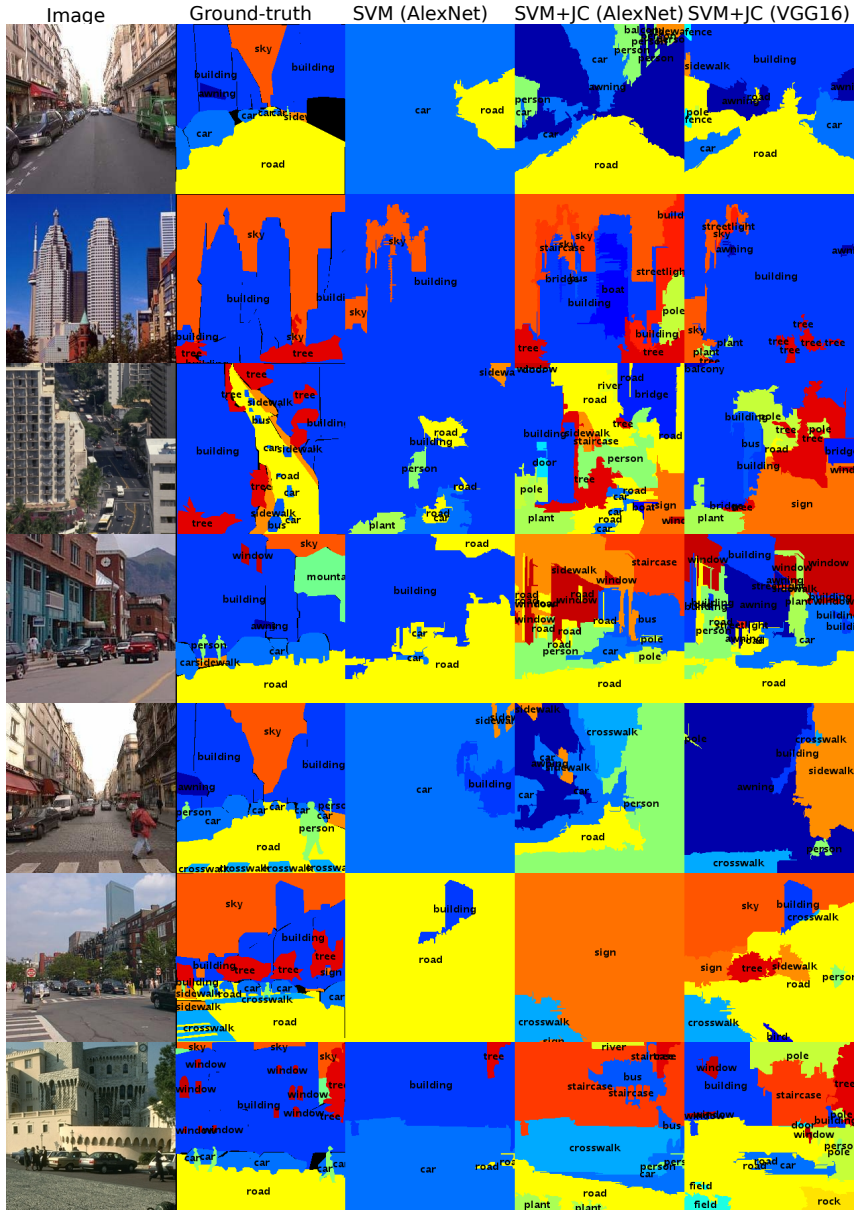
Figure 5: Weakly supervised semantic segmentation on SIFT Flow. We present uncalibrated SVM results (SVM) with AlexNet, jointly calibrated results (SVM+JC) with AlexNet, and with VGG16.
