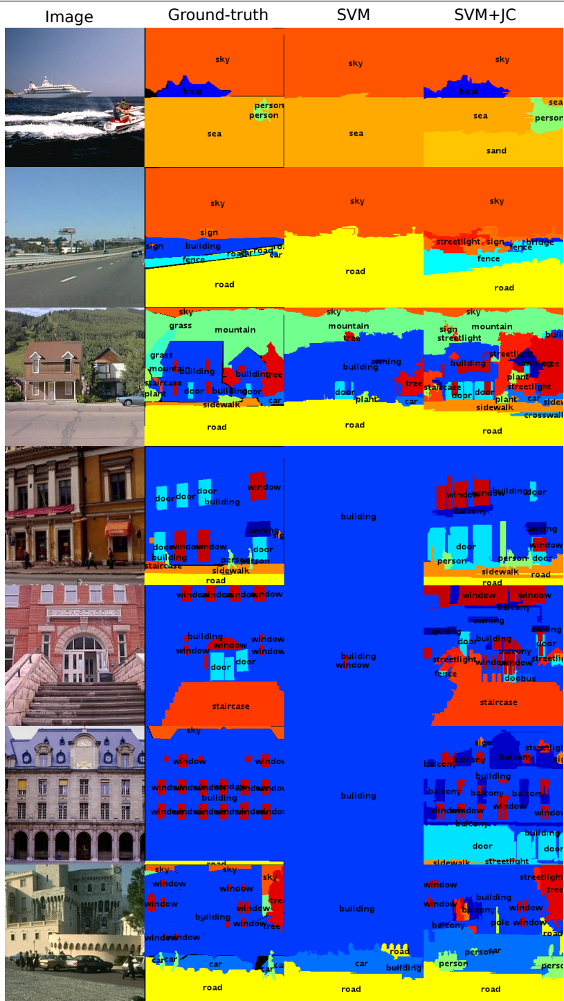
Figure 4: Fully supervised semantic segmentation on SIFT Flow. We present uncalibrated SVM results (SVM) and jointly calibrated results (SVM+JC), both with VGG16.
